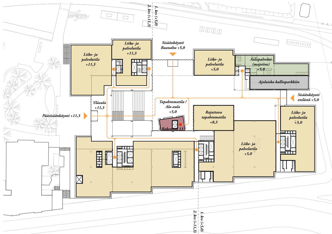
1.krs / 2.krs
