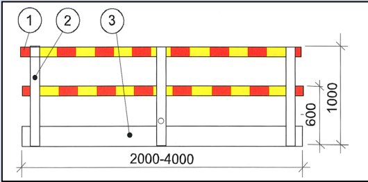
Figure 1. Example of wooden protective barrier used in light worksite protection
