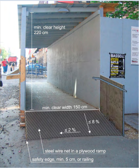
Figure 4. A temporary covered pedestrian footpath and ramp. The low wall on the right keeps pedestrians and other users from straying onto the carriageway. The steel wire net covering the plywood ramp is especially usable in wintertime conditions.
