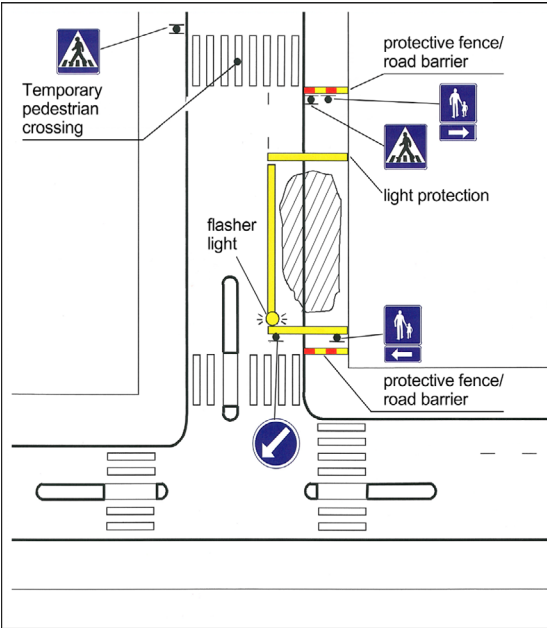
Figure 5. The protective fence/road barrier must be placed exactly at the pedestrian crossing so that persons who are partially sighted cannot miss the crossing. The middle point of the text on the signs
